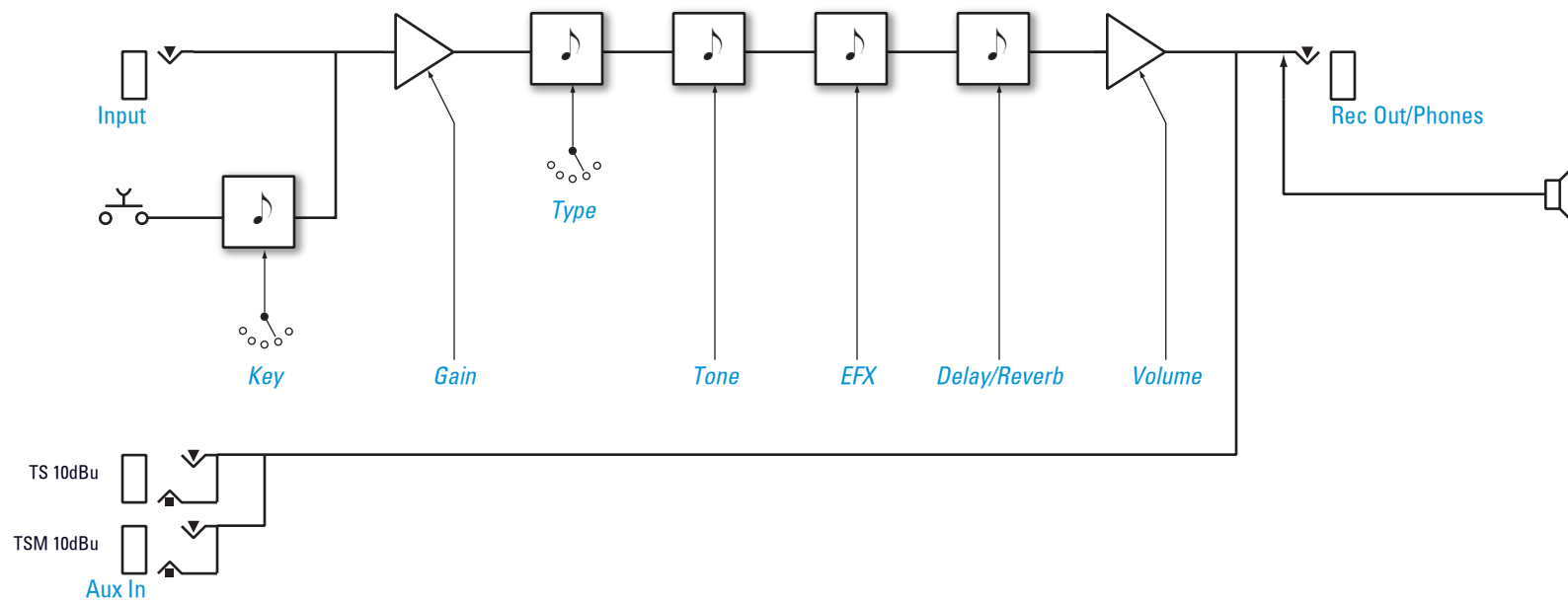
BLOCK DIAGRAM ROLAND MICRO CUBE
